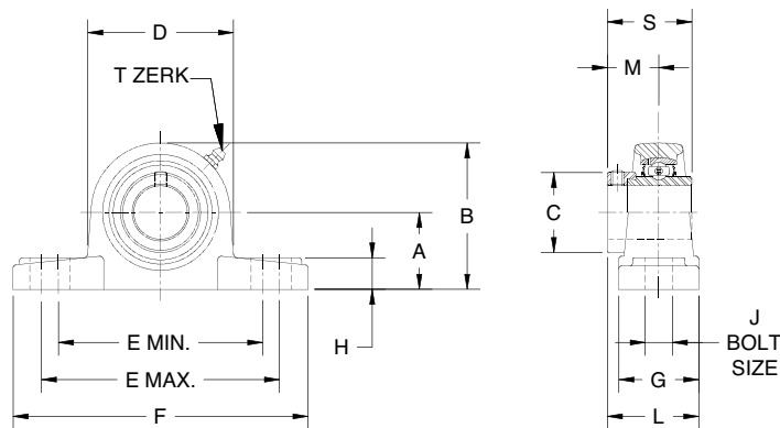
200 SERIES 2 BOLT PILLOW BLOCK ECCENTRIC LOCK – WIDE INNER RING
