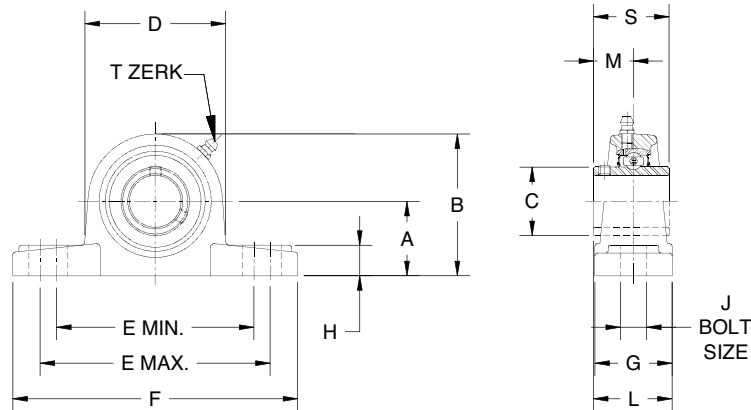
200 SERIES 2 BOLT PILLOW BLOCK SETScrew LOCK – WIDE INNER RING
