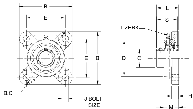
200 SERIES 4 BOLT FLANGE BLOCK SETSCREW LOCK – WIDE INNER RING
