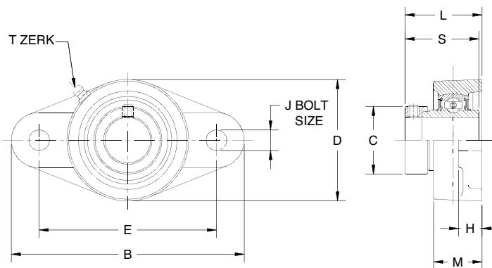
200 SERIES 2 BOLT FLANGE BLOCK ECCENTRIC LOCK – WIDE INNER RING
