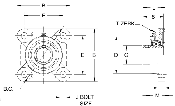
300 SERIES FLANGE BLOCK
