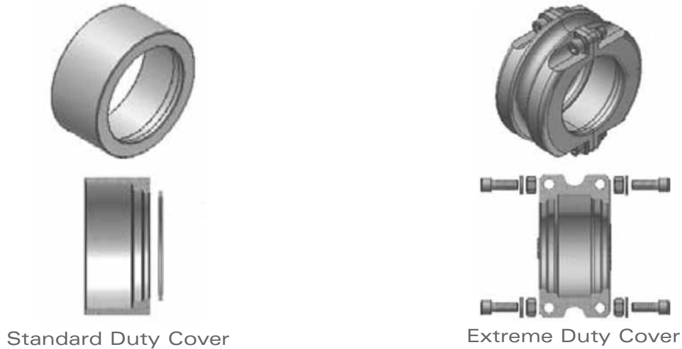
Figure 1. HUBFLEX™ covers and types, and included hardware.
