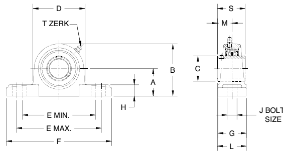
300 SERIES PILLOW BLOCK
