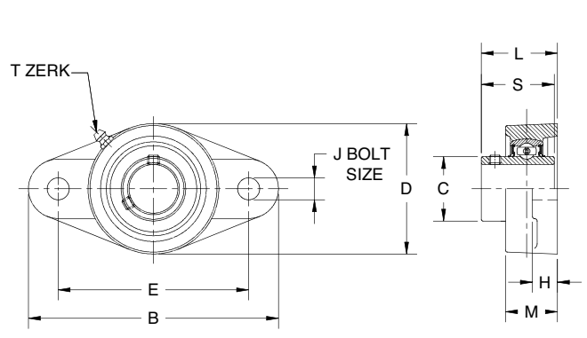
200 SERIES 2 BOLT FLANGE BLOCK SETSCREW LOCK – WIDE INNER RING
