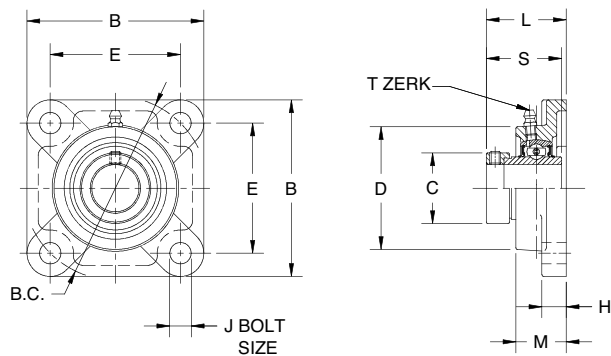
200 SERIES 4 BOLT FLANGE BLOCK ECCENTRIC LOCK – WIDE INNER RING
