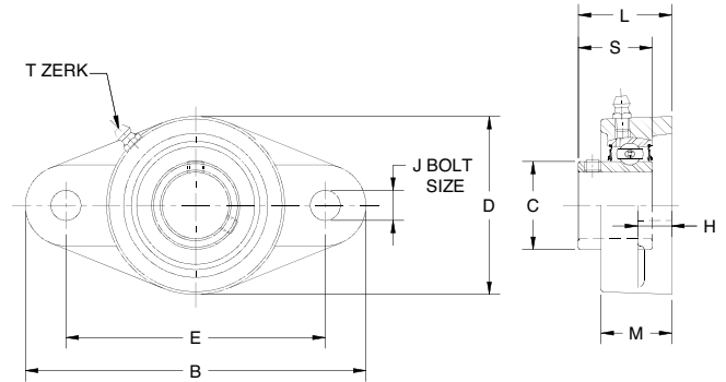
200 SERIES 2 BOLT FLANGE BLOCK SETSCREW LOCK
